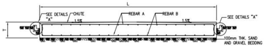
SECTION A
